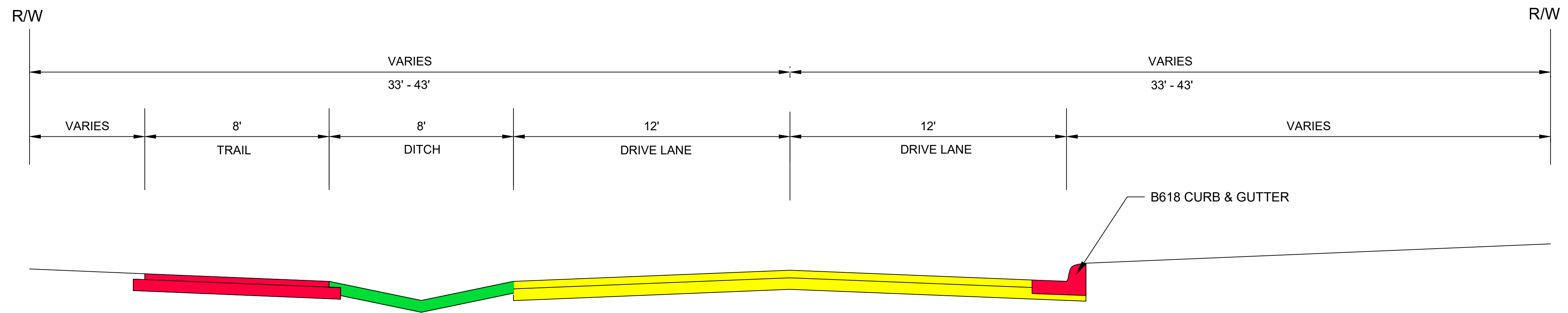
TYPICAL STREET SECTION NO CURB ALONG MIDLAND HILLS PROPERTY
