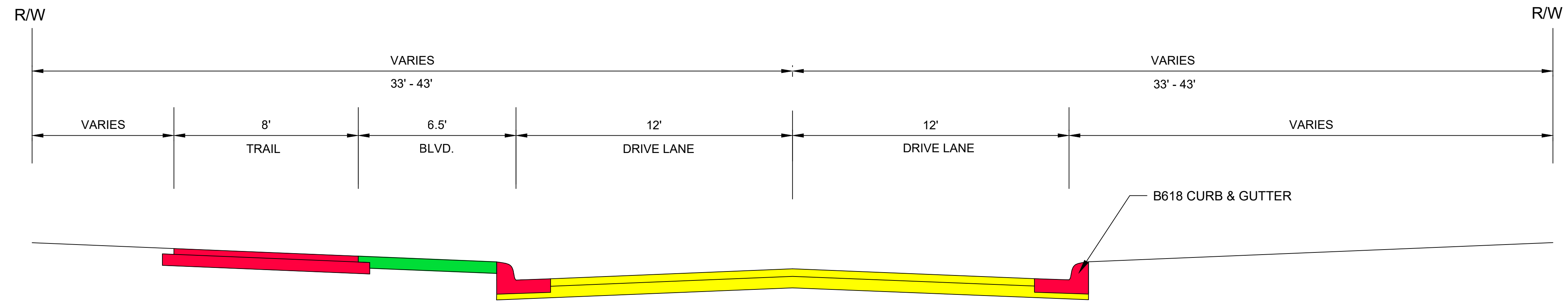
TYPICAL STREET SECTION
